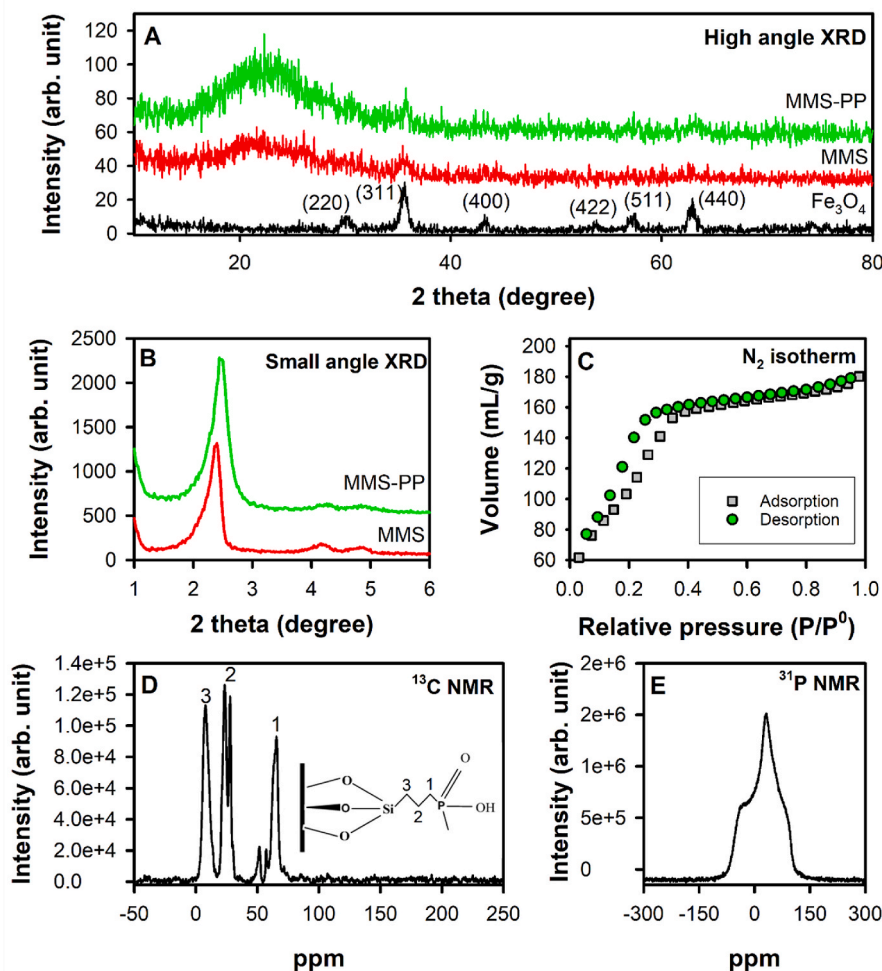
Fig. 1. Characterization of phosphonate-functionalized magnetic mesoporous silica (MMS-PP). (A) High angle powder XRD, in comparison with non-functionalized MMS and \text{Fe}_3\text{O}_4 , (B) Small angle powder XRD, in comparison with MMS, (C) \text{N}_2 adsorption-desorption isotherms, (D) ^{13}\text{C} CPMAS NMR spectrum, (E) ^{31}\text{P} CPMAS NMR spectrum.
